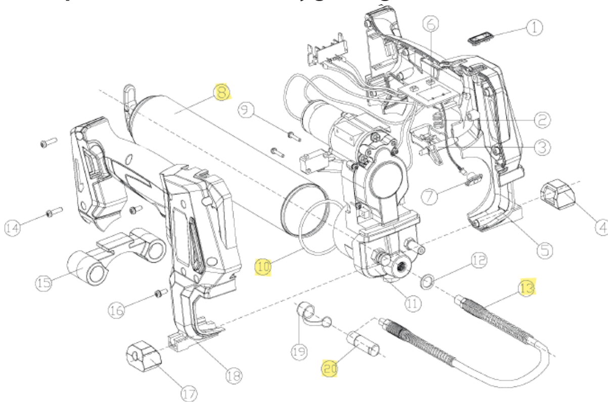
Fig. 12.-1 Exploded view of the accu grease gun
