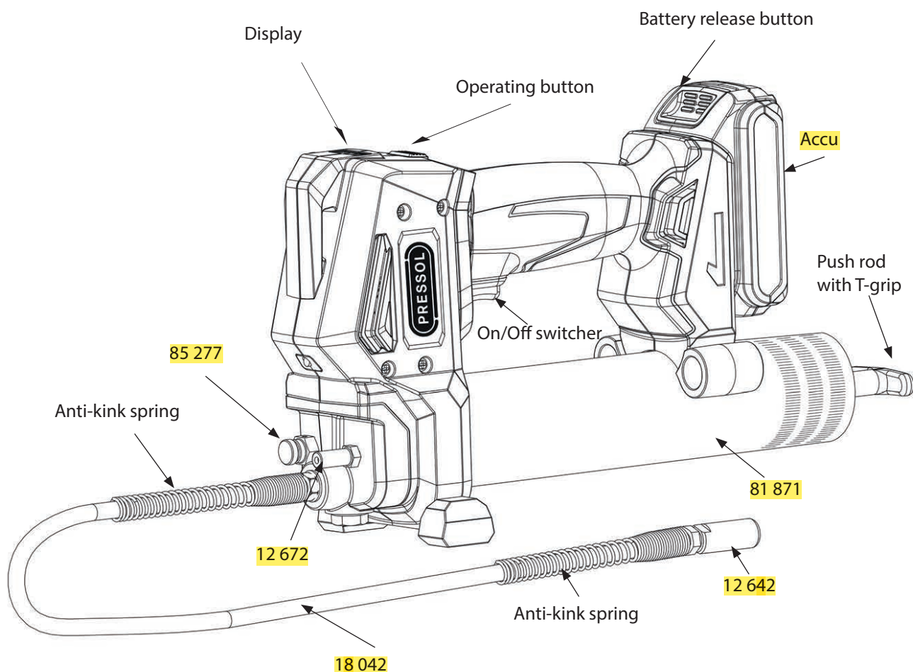
Fig. 3.2 -1: Structure battery grease gun
